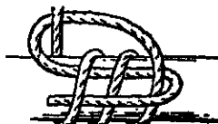
HALYARD BEND
